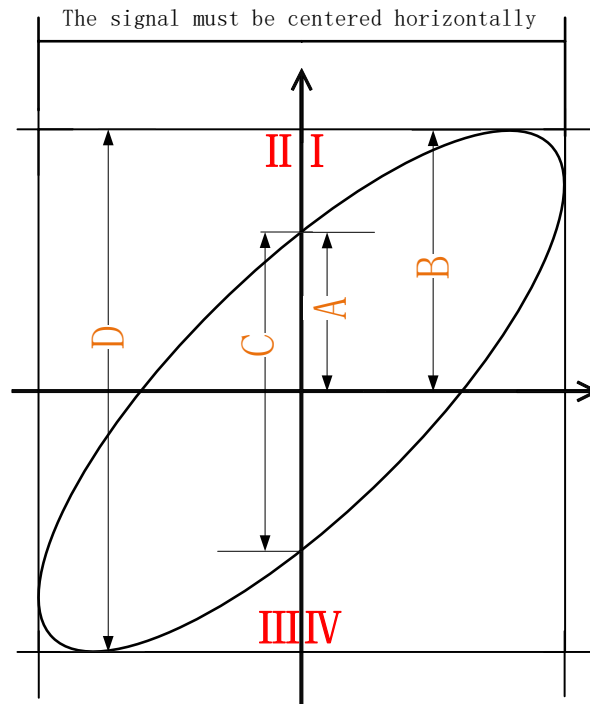
Phase difference measurement schematic
