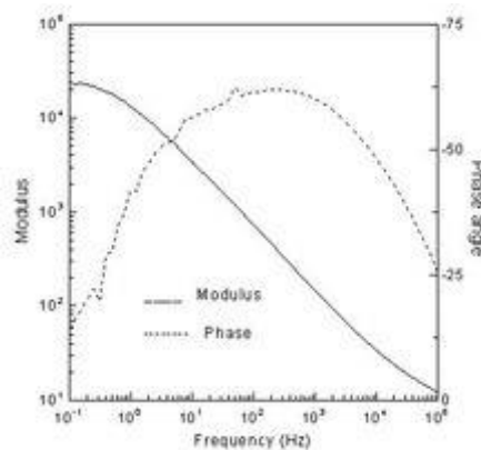
Bode plots
